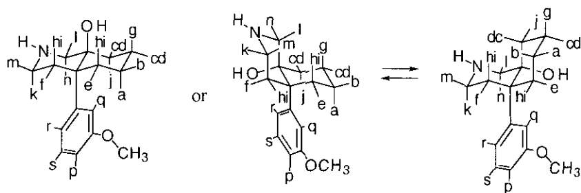
Figure 2. Possible stereostructures of compound ( 7 )
