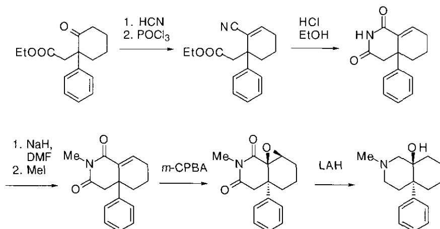
Scheme 1. Reported patent method to synthesize a 4a-aryl-8a-hydroxy- trans -decahydroisoquinoline
