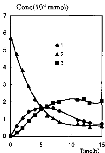
Figure 2 Photoreaction of 2
