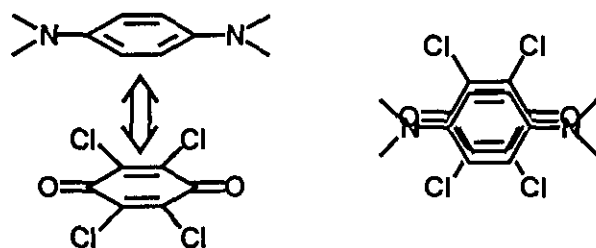
Figure III. \pi Donor - \pi acceptor complex
