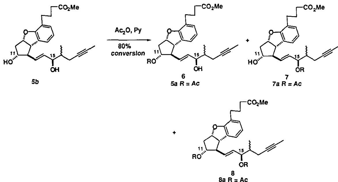
Scheme II. Acetylation of 15 \beta -hydroxy- m -phenylene \text{PGI}_2 derivative ( 5b )
