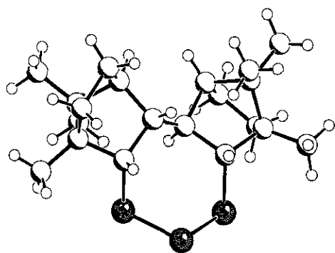
Figure 3. X-Ray crystal structure of endo,exo -(7 R ,8 S ,12 R ,13 R )-7,13,16,16,17,17-hexamethyl-9,10,11-14 R )-7,14,17,17,18,18-hexamethyl-9,10,11,12-tetrathia-trithiapentacyclo[10.2.1.1 4,7 .0 2,12 .0 3,8 ]heptadecane ( 7 ). Figure 4. X-Ray crystal structure of exo,exo -(7 R ,8 R ,13 R ,14 R )-7,14,17,17,18,18-hexamethyl-9,10,11,12-tetrathia-pentacyclo[12.2.1.1 4,7 .0 2,13 .0 3,8 ]octadecane ( 8 ).
