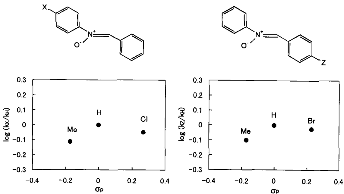
Figure 2. Plot of Hammett's sigma values ( \sigma ) versus logarithms of relative rate ratios ( \log(k_x/k_H) or \log(k_z/k_H) ).
