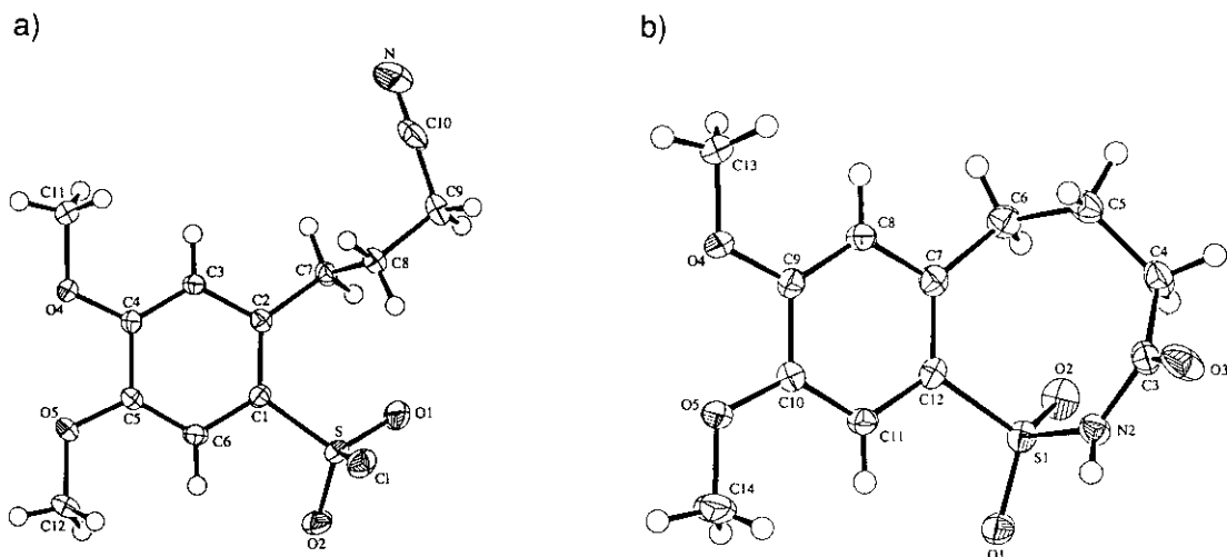
Figure 1. ORTEP plots 16 of the molecular structures of a) 7 and b) 6a (displacement ellipsoids with 50% probability).
