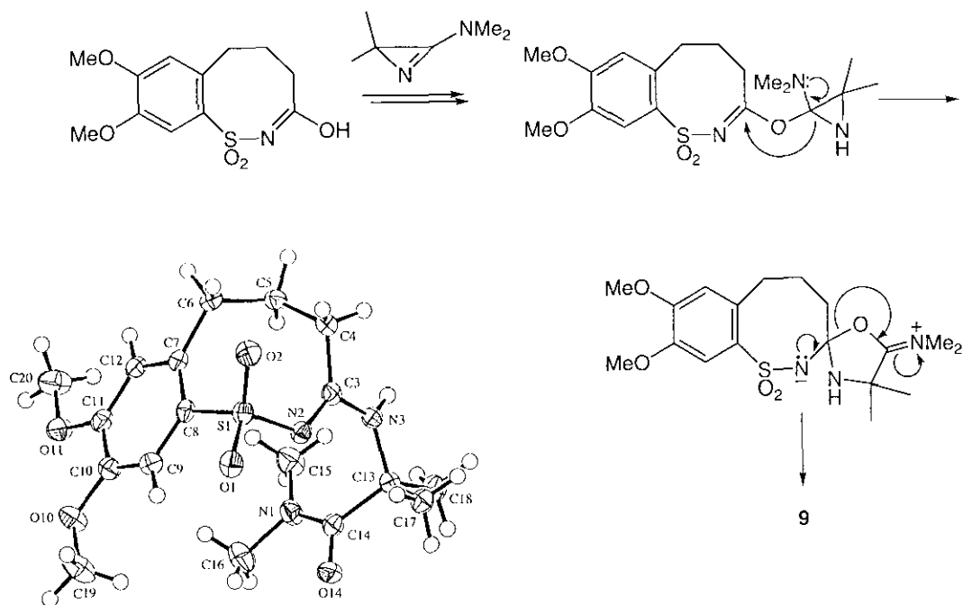
Figure 3. ORTEP plot 16 of the molecular structure of 9 (displacement ellipsoids with 50% probability).
