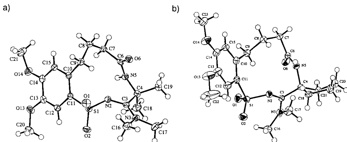
Figure 2. ORTEP plots 16 of the molecular structures of a) 8a and b) one of the independent molecules of 8c (displacement ellipsoids with 50% probability).
