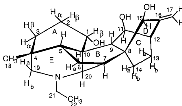
Stereostructure of lepenine 5
