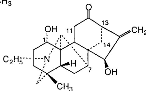
2 Songorine
