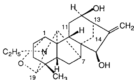
10 1,19-Dehydro-12- epi -napelline
