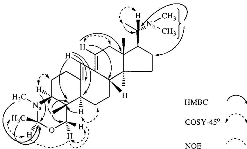
Figure 2: Important ^1\text{H} - ^1\text{H} COSY, NOE and HMBC correlations of 2 .
