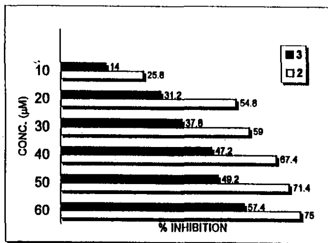
Figure 3: Effect of varying conc. of 2 and 3 on % inhibition of acetylcholinesterase.
