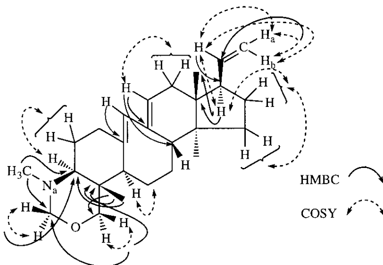
Figure 1: Important ^1H - ^1H COSY and HMBC Correlations of 1 .
