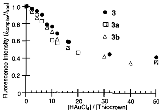
Figure 3. Dependence of fluorescence intensities of 3 , 3a , and 3b ( 2.00 \times 10^{-5} \text{ M} ) at 364 nm on concentration of \text{H[AuCl}_4\text{]} .
