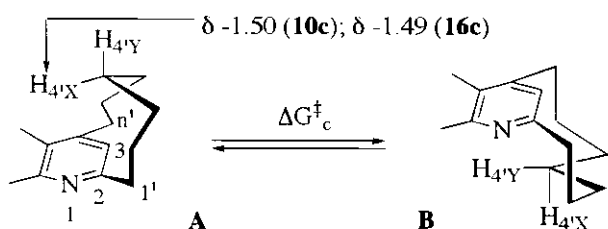
Figure 2 The flipping of the heptamethylene bridge of 10c and 16c
