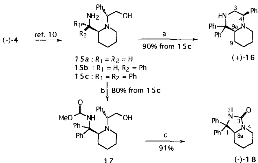
Scheme 2 : (a) \text{MsCl} , \text{Et}_3\text{N} , \text{CH}_2\text{Cl}_2 , rt, 1 h; (b) \text{ClCO}_2\text{Me} , aq. 15% \text{NaOH} , \text{CHCl}_3 , rt, 3 h; (c) \text{H}_2 , 10% \text{Pd/C} , MeOH, 12 h
