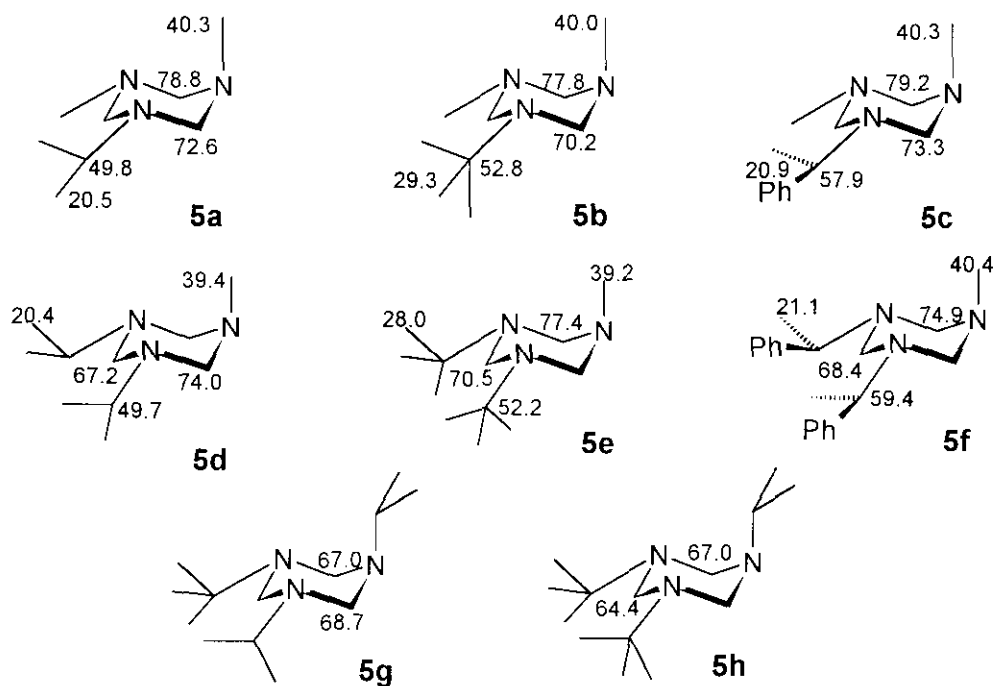
Scheme 6 ^{13}\text{C} NMR chemical shifts of non-symmetrically N -substituted triazines ( 5a-h )
