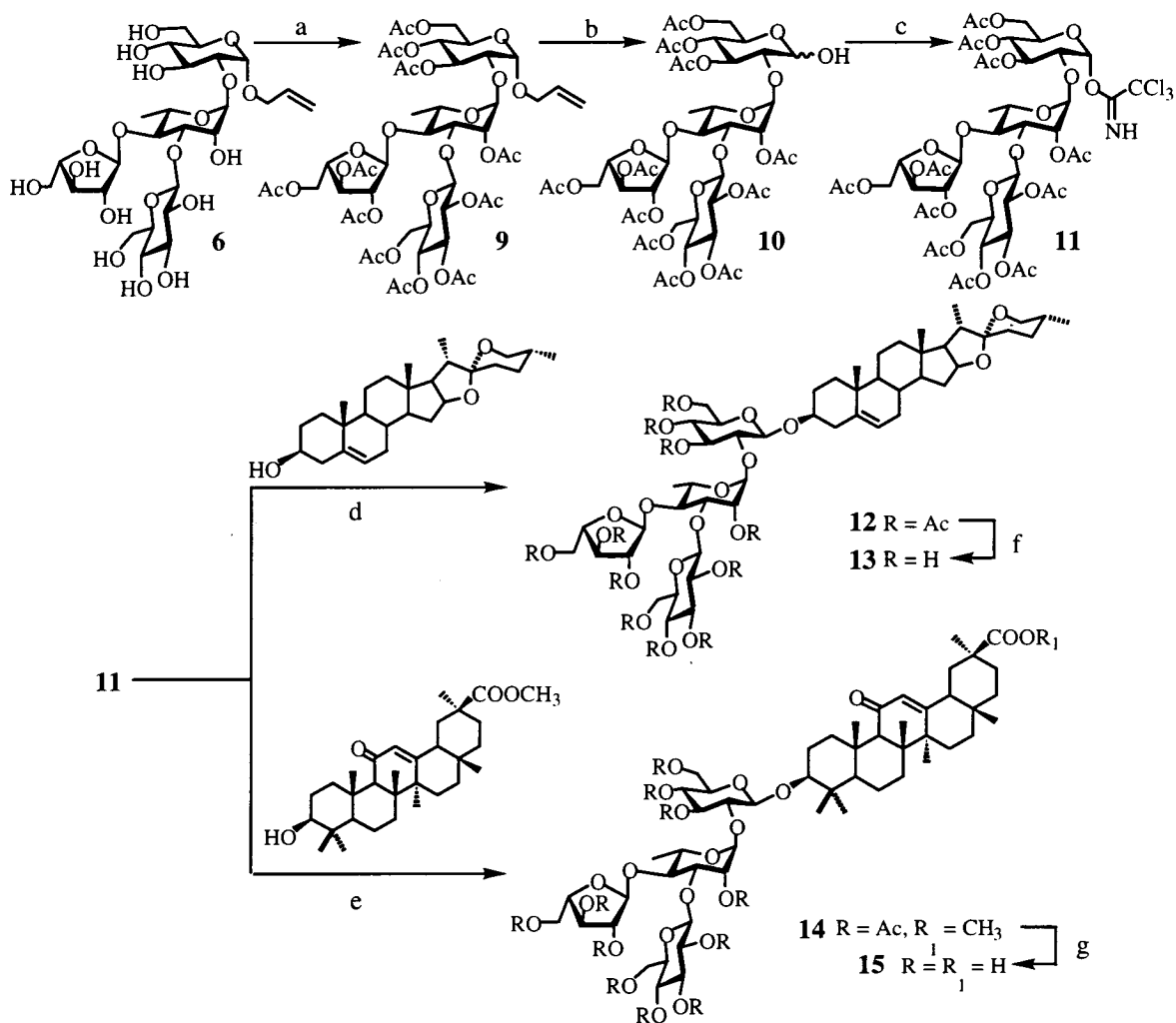
Scheme 3. Reagents and Conditions: a) \text{Ac}_2\text{O} , pyridine, rt, 52 h, 82 %; b) \text{Pd}[\text{P}(\text{Ph})_3]_4 , 80 °C, 1 h, quantitative; c) \text{CCl}_3\text{CN} , DBU, \text{CH}_2\text{Cl}_2 , 0 °C, 2 h, 94 %; d) diosgenin, MS 4 Å, \text{BF}_3 \cdot \text{Et}_2\text{O} , \text{CH}_2\text{Cl}_2 , -10 °C, 4 h, 66 % ( \alpha : \beta ; 1 : 4); e) methylglycyrrhetinate, MS 4 Å, \text{BF}_3 \cdot \text{Et}_2\text{O} , \text{CH}_2\text{Cl}_2 , -20 °C, 4 h, 70 % ( \alpha : \beta ; 1 : 3); f) 1N NaOH-EtOH (1:1), rt, 8 h, 94 %; g) 1N NaOH-EtOH (1:1), reflux, 8 h, 97 %.
