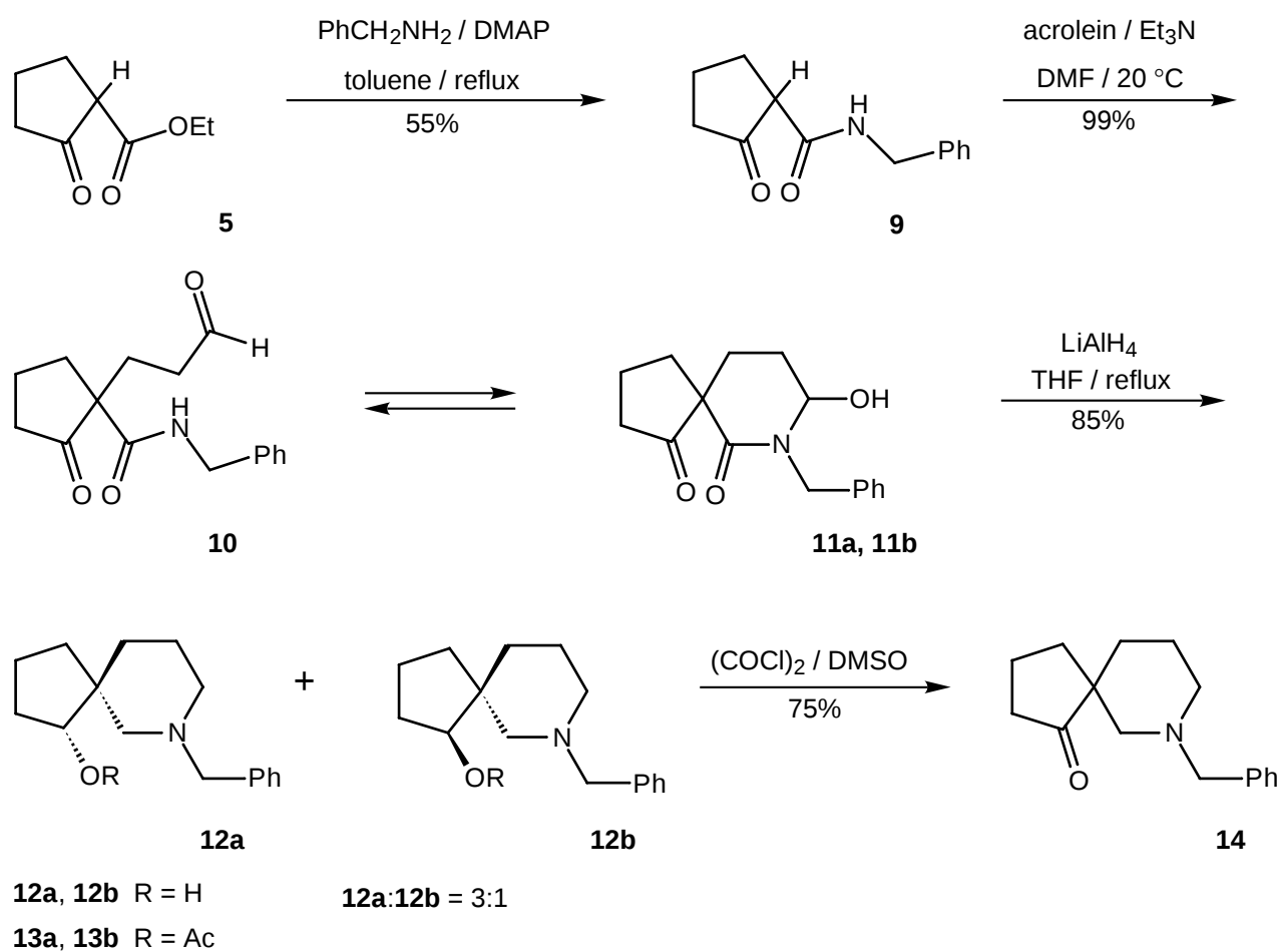
Scheme 3. Four step synthesis of spirocyclic ketone ( 14 ) from \beta -keto ester ( 5 ).
