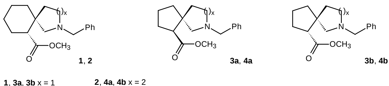
Scheme 1. GABA-analogous amino acid esters based on spirocyclic ring systems.
