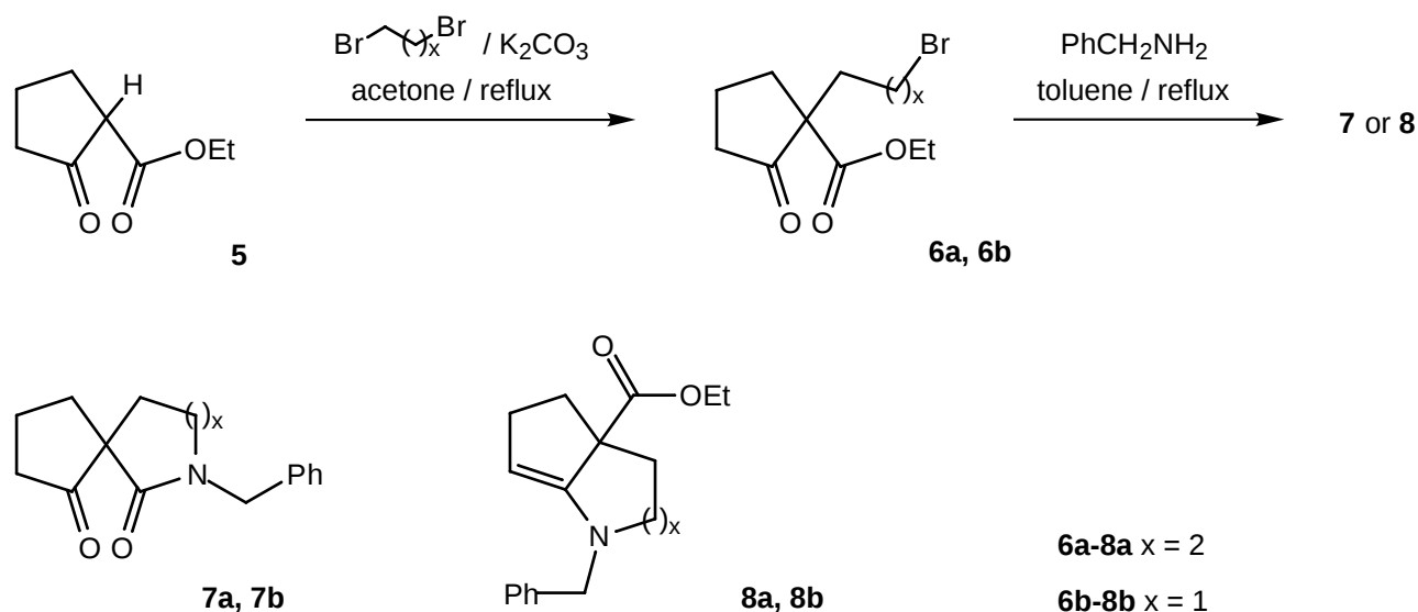
Scheme 2. Cyclization of bromoalkyl substituted \beta -keto esters ( 6a and 6b ) with benzylamine.
