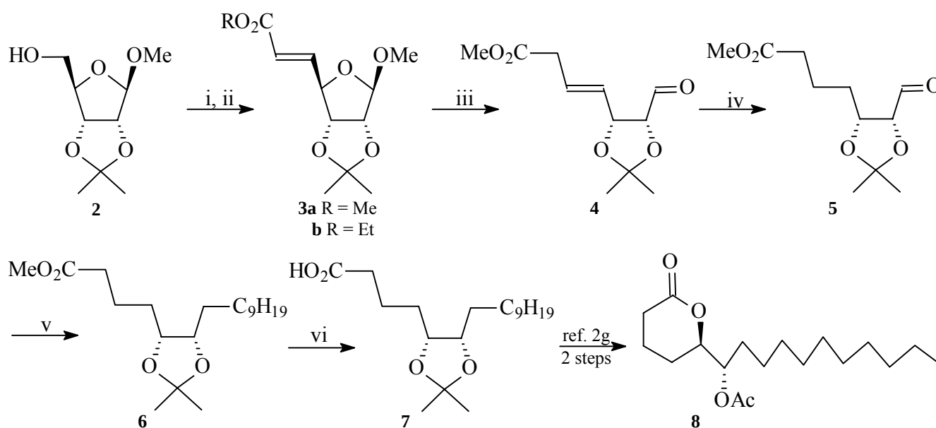
Scheme 1 Reagents and Conditions: i, \text{CrO}_3 , dry pyridine, \text{CH}_2\text{Cl}_2 , 20 °C, 20 min; ii, \text{Ph}_3\text{P}=\text{CHCO}_2\text{R} (R = Me or Et), \text{PhCO}_2\text{H} (10%), \text{CH}_2\text{Cl}_2 , 20 °C, 12 h, 65-70% from 2 , E/Z ca. 10/1; iii, 0.15 M solution of 3 in MeOH, Mg (10 equiv.), 0 °C, 1 h, 52% (40% recovered); iv, \text{H}_2 , 10% Pd/C, MeOH, 20 °C, 30 min 86%; v, (a) \text{Ph}_3\text{P}^+(\text{CH}_2)_8\text{MeBr}^- , 1.6 M n -Buli in pentane, -78 °C, THF, (b) \text{H}_2 , 10% Pd/C, MeOH, 20 °C, 1 h, 42% overall; vi, 10% aqueous KOH, MeOH, 20 °C, 2 h, 90%.
