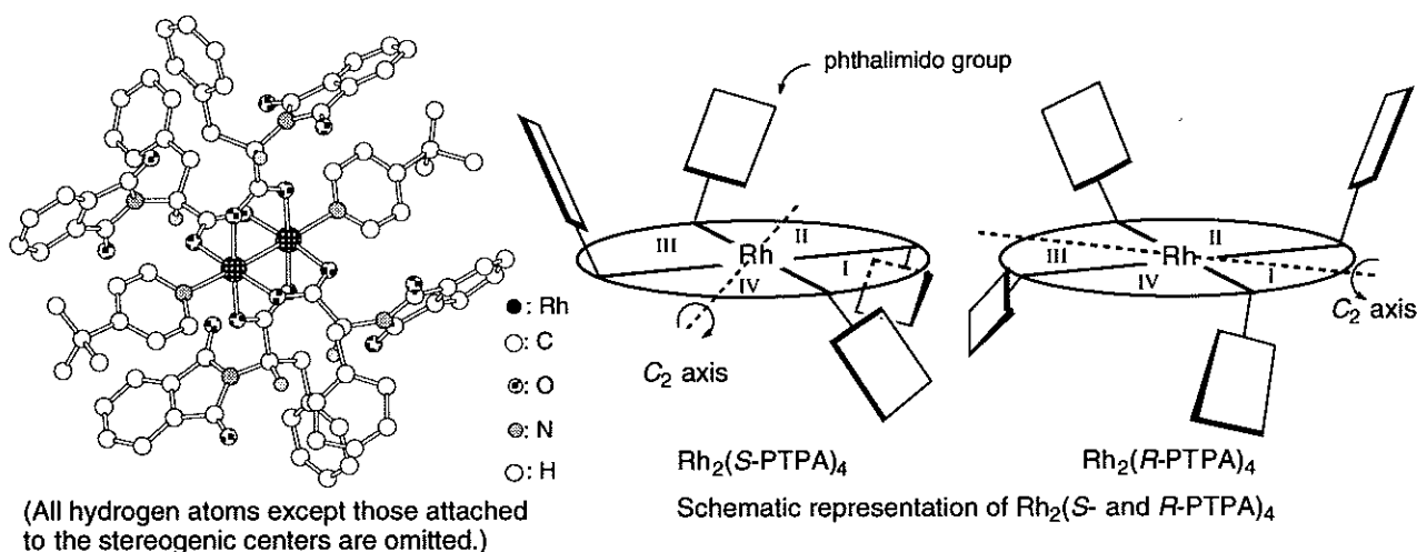
Figure 1. Crystal structure of bis(4- tert -butylpyridine) adduct of \text{Rh}_2(\text{S-PTPA})_4
