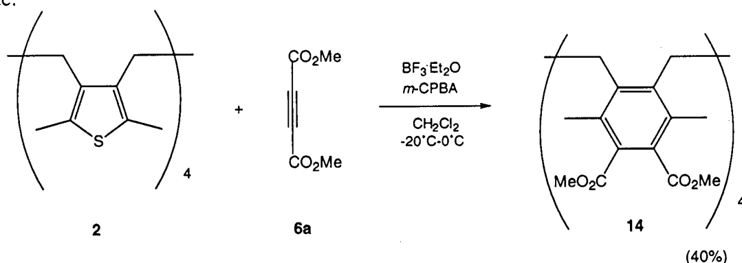
Scheme 9 Quadruple Cycloaddition Using \text{BF}_3 \cdot \text{Et}_2\text{O} as Lewis Acid
