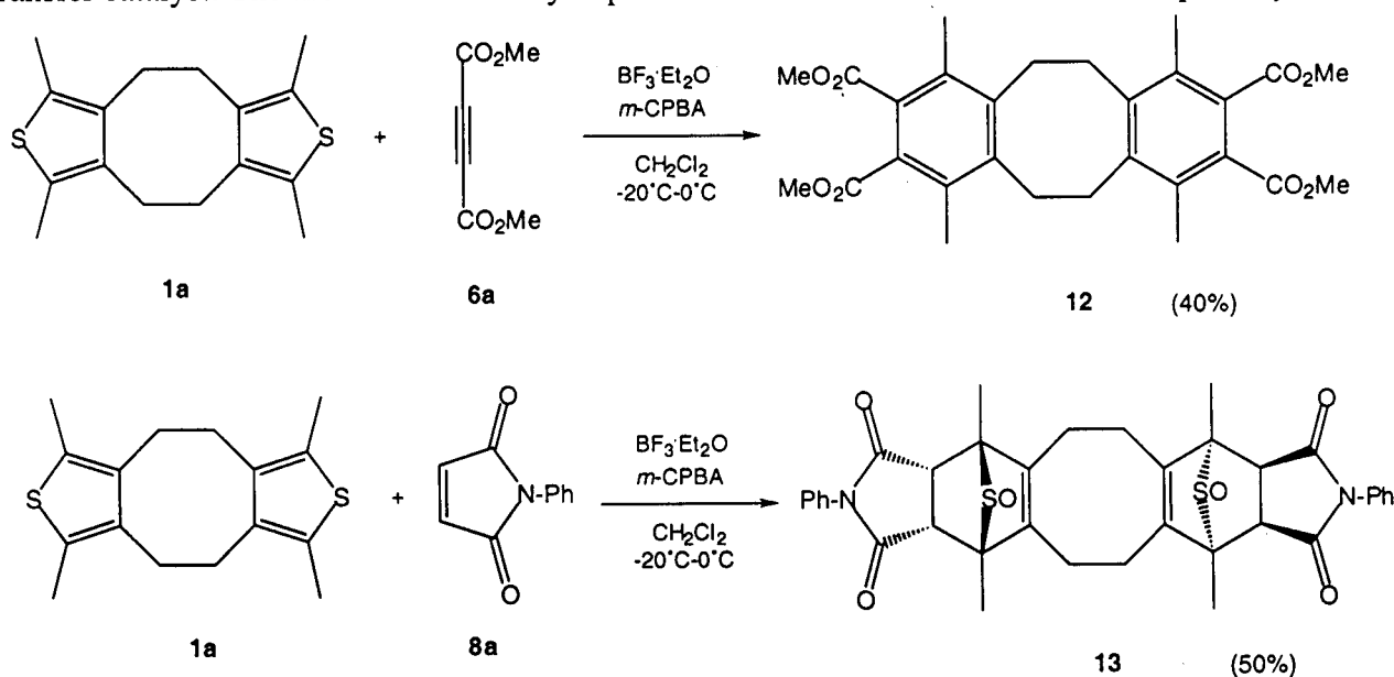
Scheme 8 Double Cycloaddition Using \text{BF}_3 \cdot \text{Et}_2\text{O} as Lewis Acid
