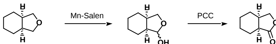
Scheme 1. Oxidative desymmetrization of meso compounds
