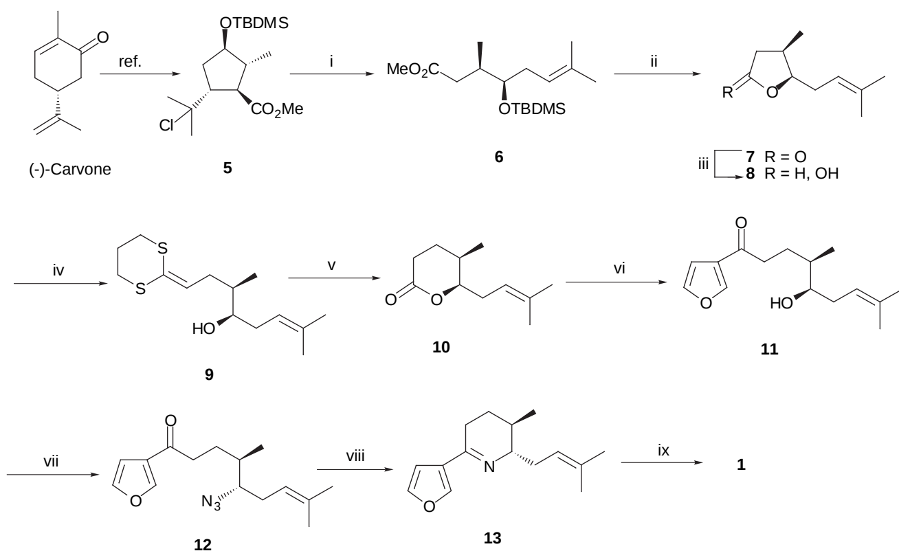
Scheme 1 Reagents and conditions: i, 3.7 eq. Sm, 3.5 eq. 1,2-diiodoethane, THF-HMPA (20:1), rt (85.5%); ii, Bu 4 NF, THF, rt; iii, DIBAL, THF, -78°C (97.2% from 6 ); iv, 2-trimethylsilyl-1,3-dithiane, n -BuLi, THF, -15°C; v, p -TsOH, CH 2 Cl 2 , rt (69.5% from 8 ); vi, 3-bromofuran, n -BuLi, THF, -78°C (92.1%); vii, Ph 3 P, DEAD, (PhO) 2 P(O)N 3 , THF, 0°C; viii, Ph 3 P, THF, reflux; ix, NaBH 4 , EtOH, rt (77.4% from 12 ).
