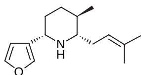
1 (-)-Anhydronupharamine
