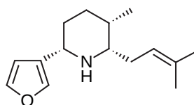
3 (-)-Nuphenine
