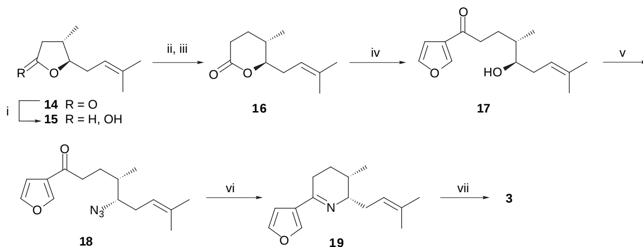
Scheme 2 Reagents and conditions: i, DIBAL, THF, -78°C; ii, 2-trimethylsilyl-1,3-dithiane, n -BuLi, THF, -15°C; iii, p -TsOH, \text{CH}_2\text{Cl}_2 , rt (90.5% from 15 ); iv, 3-bromofuran, n -BuLi, THF, -78°C (98.0%); v, \text{Ph}_3\text{P} , DEAD, (\text{PhO})_2\text{P}(\text{O})\text{N}_3 , THF, 0°C (80.5%); vi, \text{Ph}_3\text{P} , THF, reflux; vii, \text{NaBH}_4 , EtOH, rt (73.4% from 18 ).
