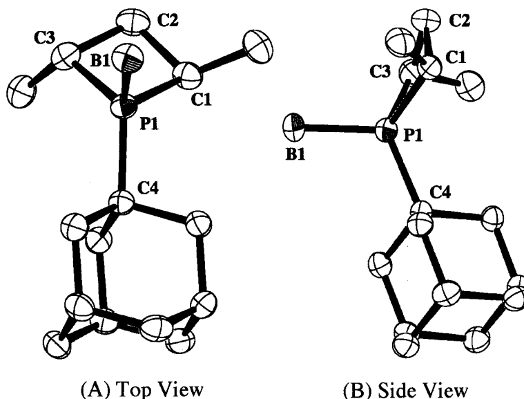
Figure 1. ORTEP drawing of ( R,R )- 3a . Crystal Data: \text{C}_{15}\text{H}_{28}\text{BP} , orthorhombic, space group \text{P2}_1\text{2}_1\text{2}_1 ; bond lengths \text{P1-B1} 1.922(5) Å, \text{P1-C1} 1.838(4) Å, \text{P1-C3} 1.851(5) Å, \text{P1-C4} 1.840(4) Å; bond angles \text{C1-P1-C3} 79.3(2)^\circ , \text{C1-C2-C3} 99.4(3)^\circ , \text{P1-C1-C2} 88.5(3)^\circ ,
