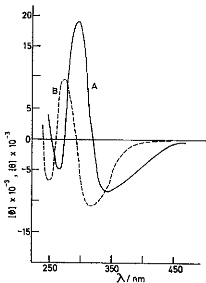
Figure 3 O.r.d. (A) and c.d. (B) curves of natural O-methylandrocybine ( in methanol )
