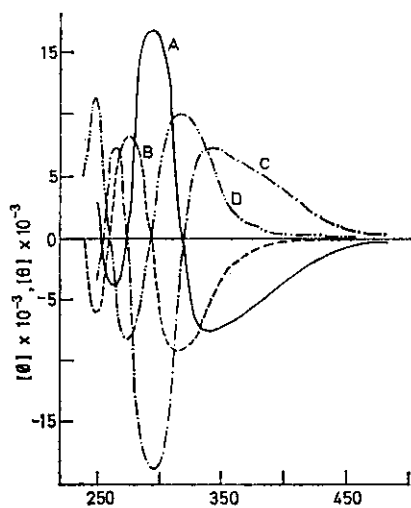
Figure 2 O.r.d. (A) and c.d. (B) curves of (-)-O-methylandrocybine ( IIA ) and o.r.d. (C) and c.d. (D) curves of (+)-O-methylandrocybine ( IIB ) ( in methanol )
