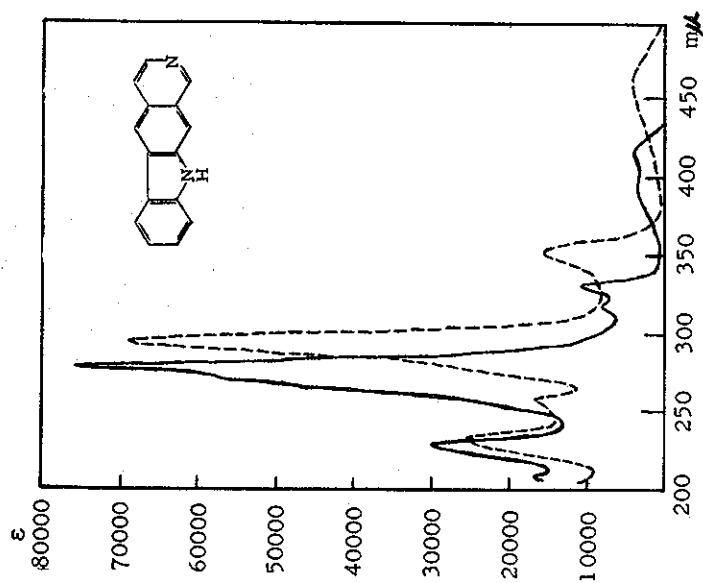
Fig. 1 6H-Pyrido[3,4-b]carbazole
