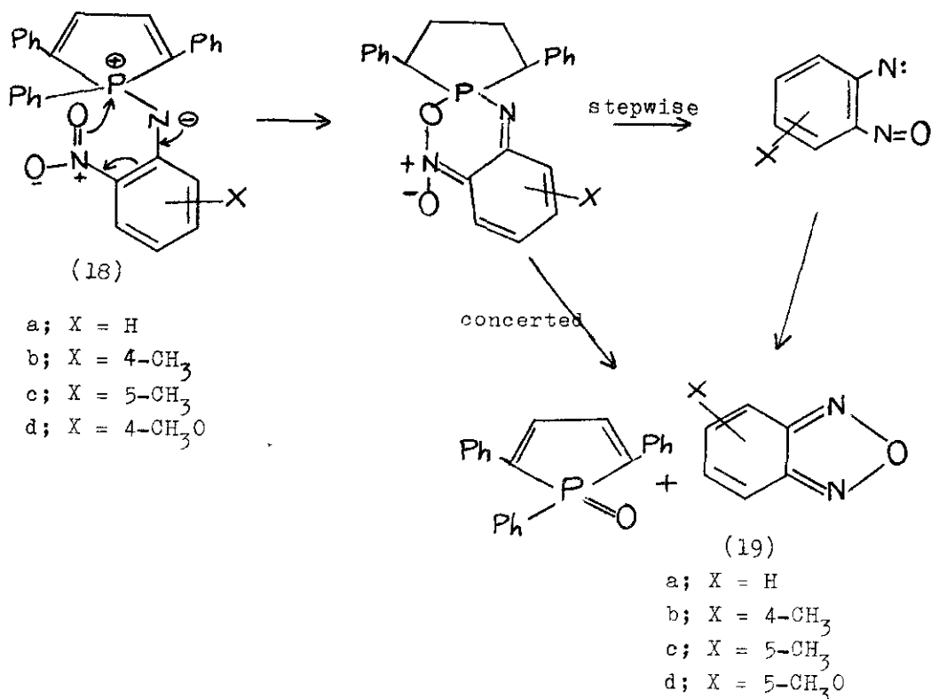
Scheme 3.
