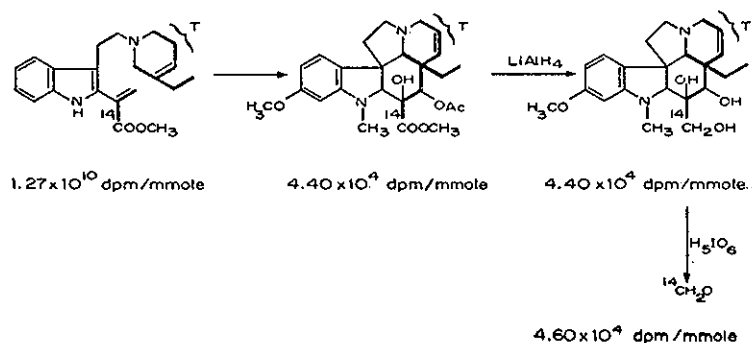
Figure 8. Degradation of vindoline from [ 14 COOCH 3 , 3,14,15,21- 3 H]-secodine.
