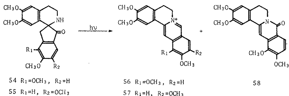
Scheme 9
