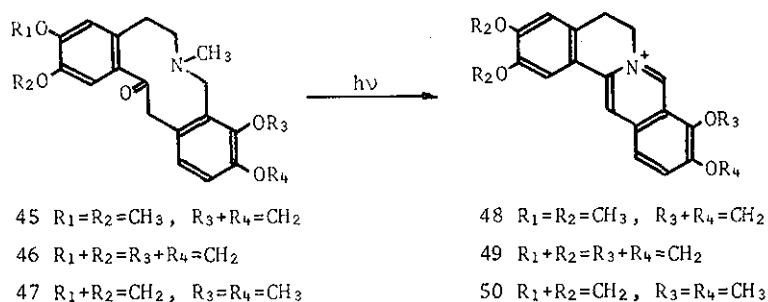
Scheme 7
