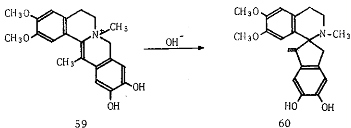
Scheme 10
