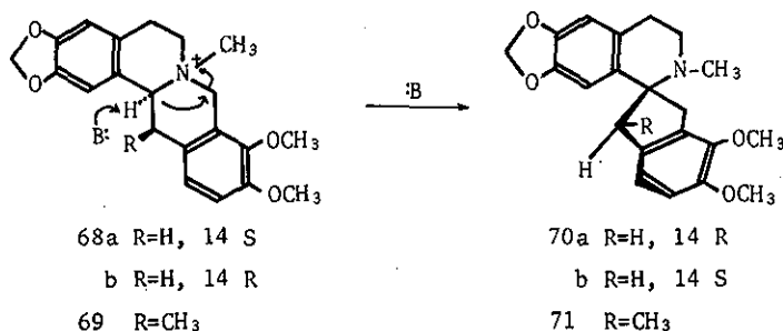
Scheme 12
