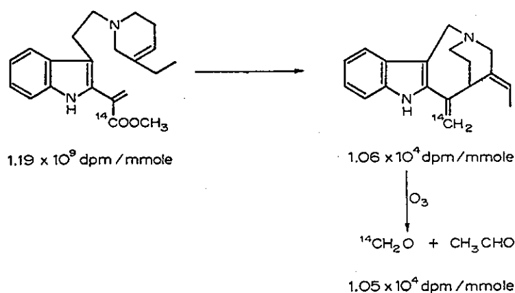
Figure 4. Degradation of apparicine from incorporation of [^{14}\text{COOCH}_3] -secodine.
