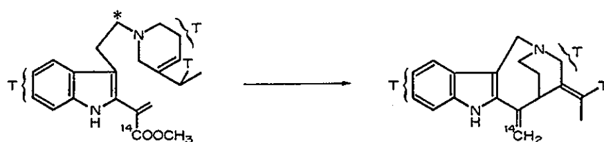
Figure 6. A summary of results involving incorporation of secodine into apparicine in A. pyricollum .
