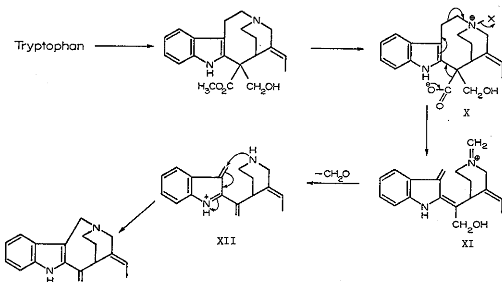
Figure 7. The Potier postulate for the conversion of stemmadenine to apparicine.
