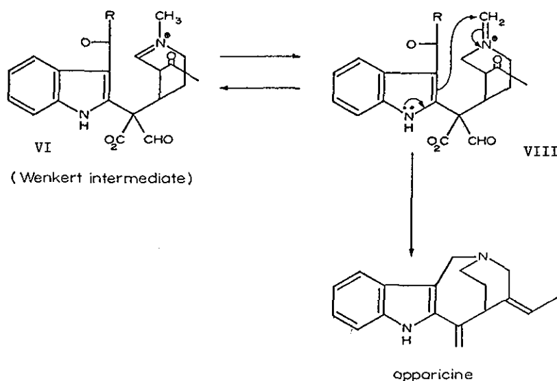
Figure 2. Djerassi-Gilbert postulate for apparicine.
