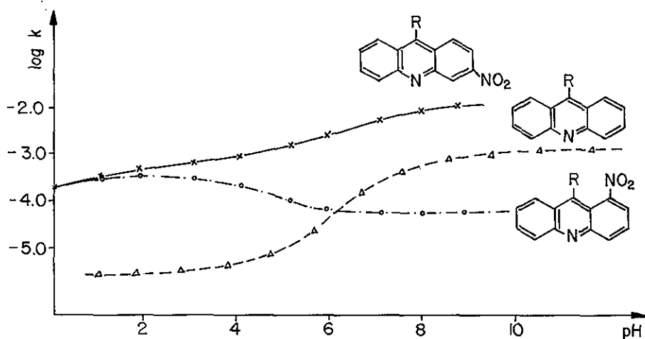
Fig.1. Plots of log k versus pH for C-137 (----), C-257 (—), and C-283 (— · —); R = \text{NH}(\text{CH}_2)_3\text{N}(\text{CH}_3)_2 .
