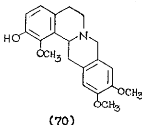
Scheme 28
