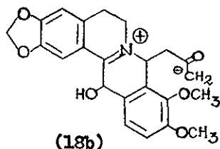
Scheme 20
