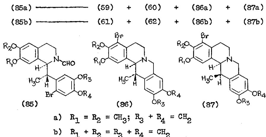
Scheme 38
