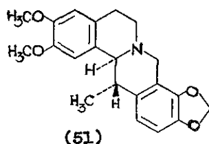
Scheme 23
