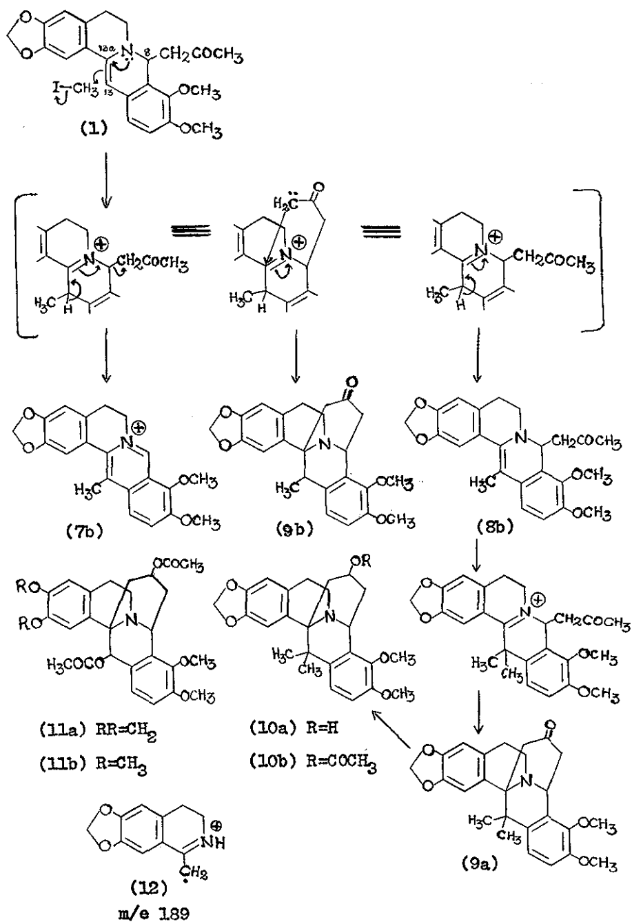
Scheme 6
