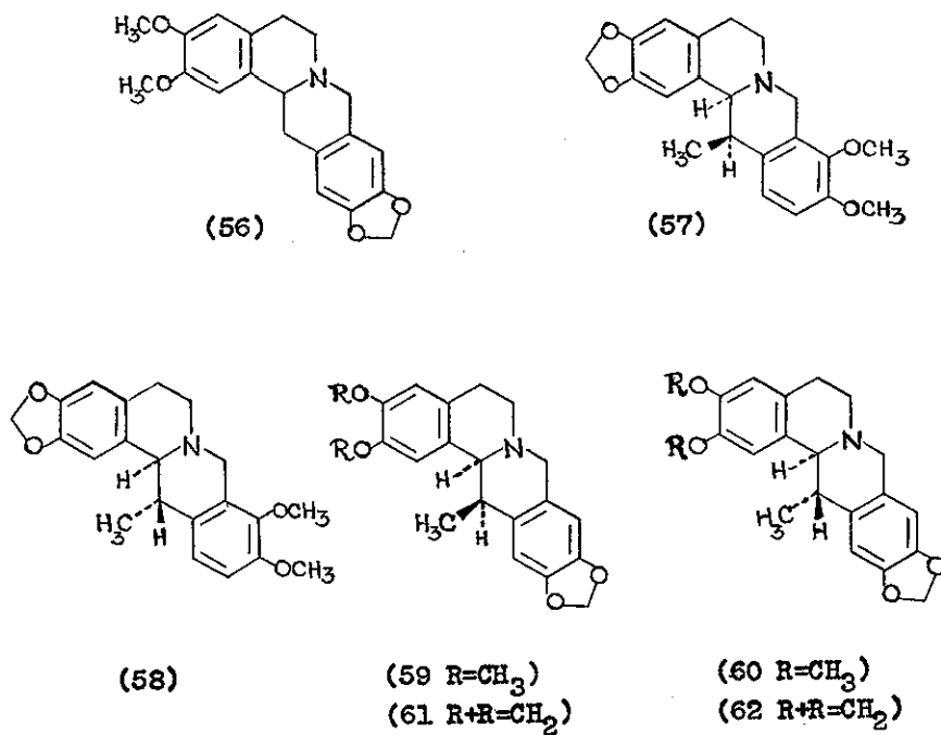
Scheme 26
