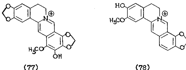
Scheme 33
