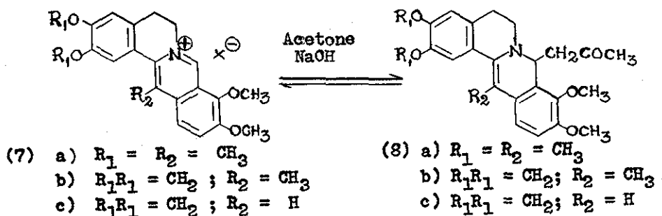
Scheme 5
