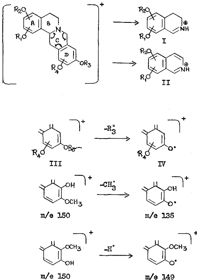
Scheme 34
