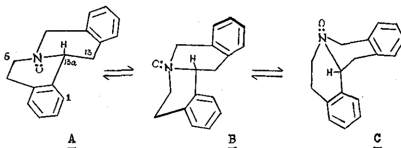
Scheme 21
