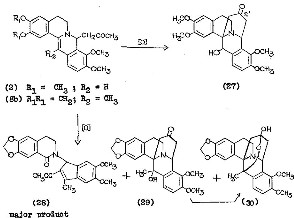
Scheme 14
