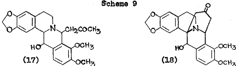
Scheme 9
