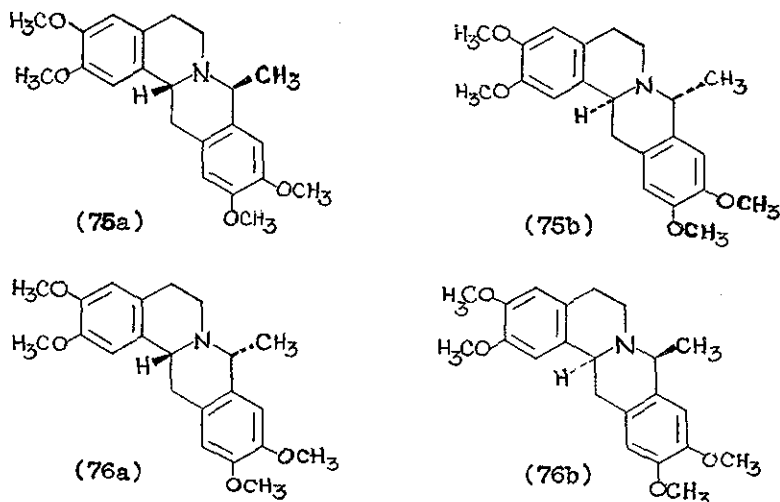
Scheme 32
