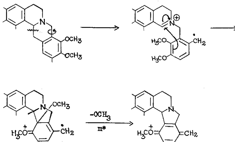
Scheme 35
