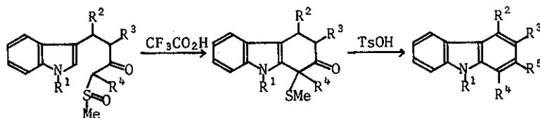
7, R 1 =R 2 =R 3 =R 4 =H 8, R 1 =Me, R 2 =R 3 =R 4 =H 9, R 1 =CH 2 Ph, R 2 =R 3 =R 4 =H 10, R 1 =Me, R 2 =R 4 =H, R 3 =NHAc 11, R 1 =R 2 =R 3 =H, R 4 =Me 12, R 1 =R 2 =R 4 =H, R 3 =Me 13, R 1 =CH 2 Ph, R 2 =Me, R 3 =R 4 =H, 20
