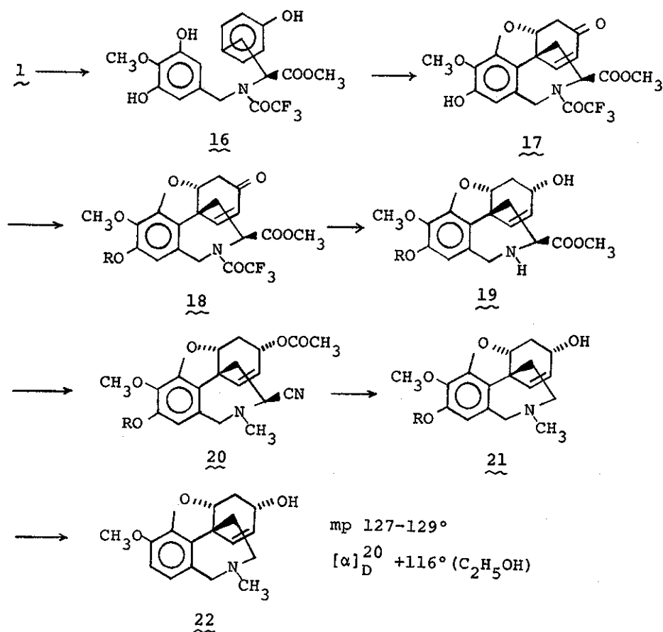
Chart 3 \text{R} = (\text{C}_2\text{H}_5\text{O})_2\text{PO}
