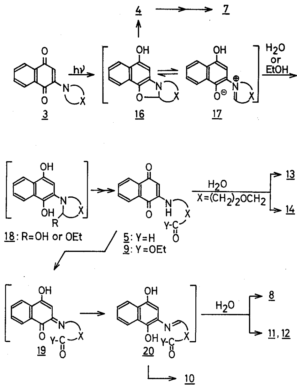
Scheme I
