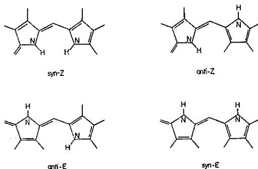
Fig.3 Configuration of dipyrromethenes
