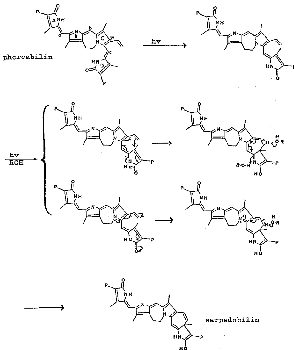
Fig.7 Proposed mechanism for the isomerisation of phorcabilin into sarpedobilin ( \text{P}=\text{CH}_2\text{CH}_2\text{COOR} ; \text{R}=\text{H} or \text{CH}_3 )
