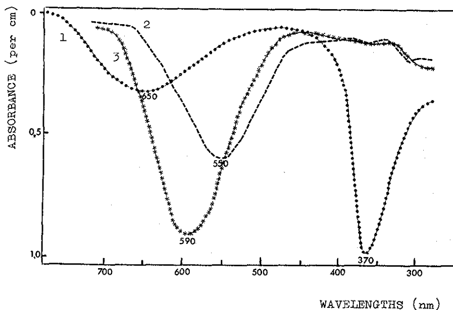
Fig. 6 Absorption spectra in MeOH of: (1) pterobilin ester (2) phorbabilin ester (3) sarpedobilin ester
