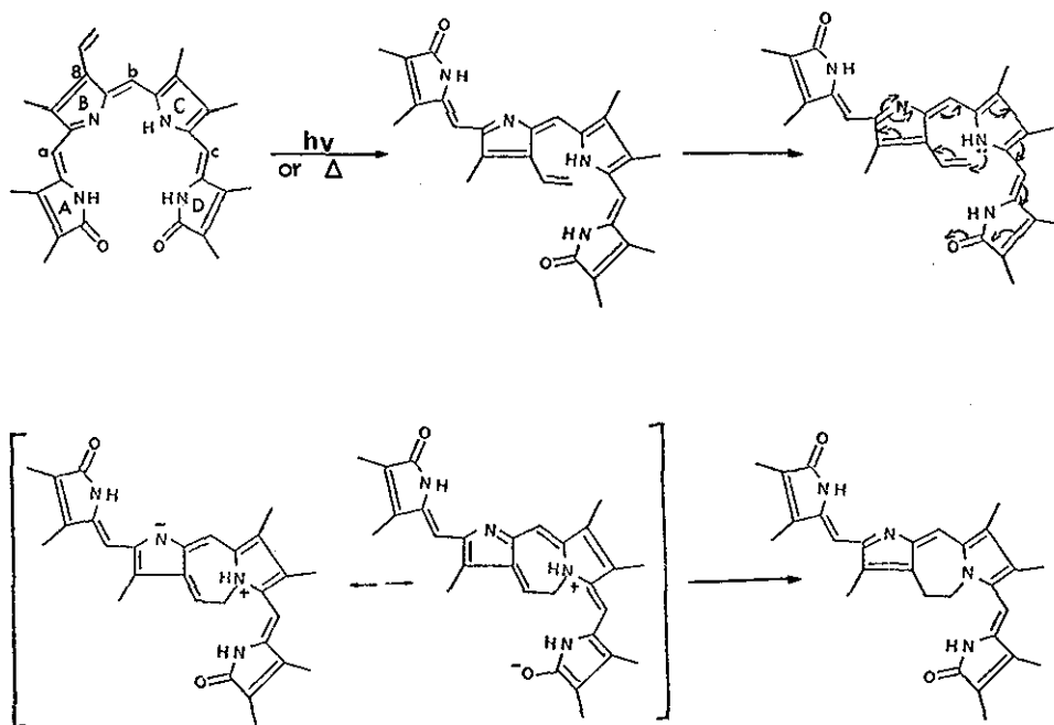
Fig.5 Proposed mechanism for the cyclisation of biliverdins IX \beta or IX \delta
