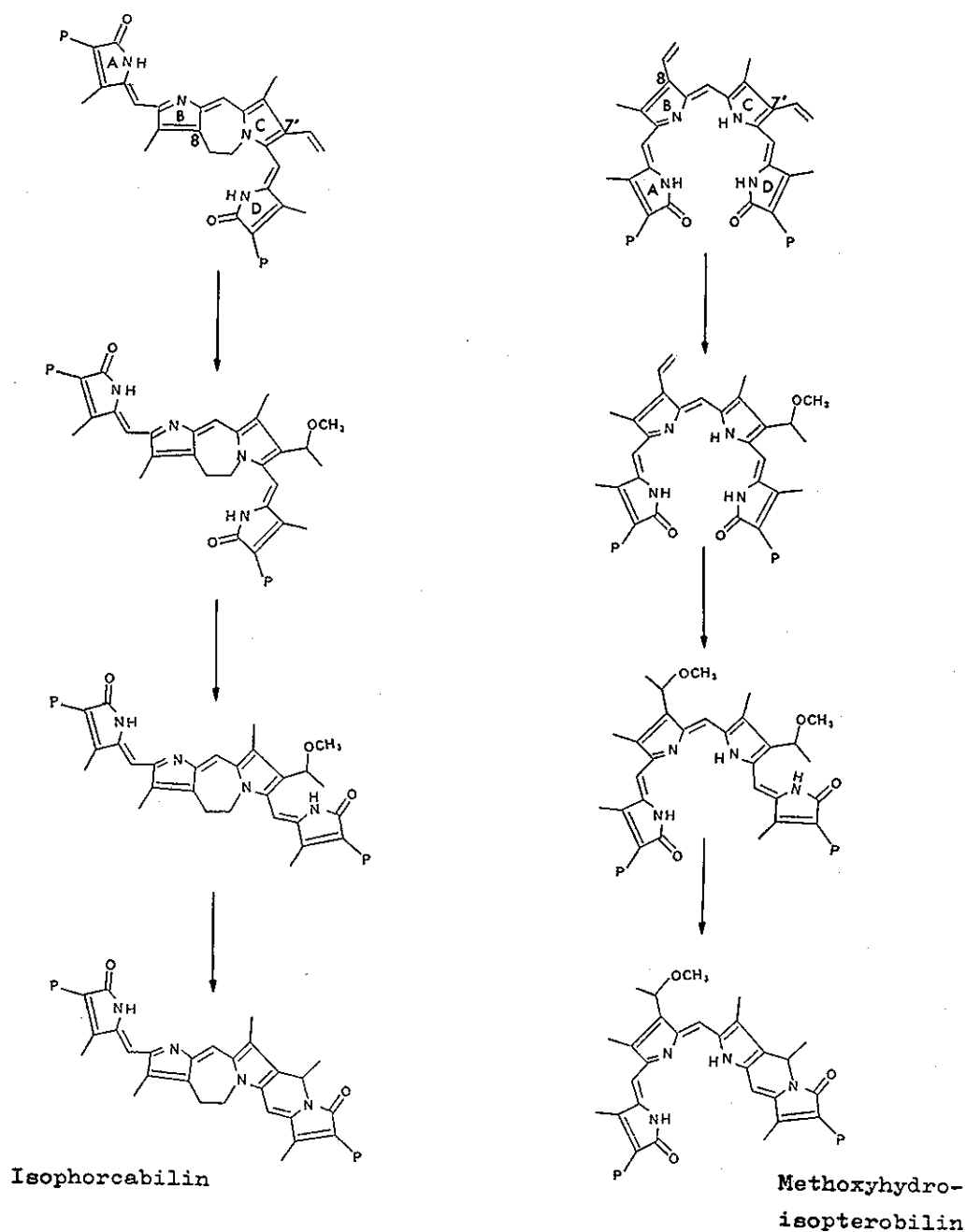
Fig.8 Reactions of phorcabilin and pterobilin in MeOH/H + (P=CH 2 CH 2 COOR, R=H or CH 3 )
