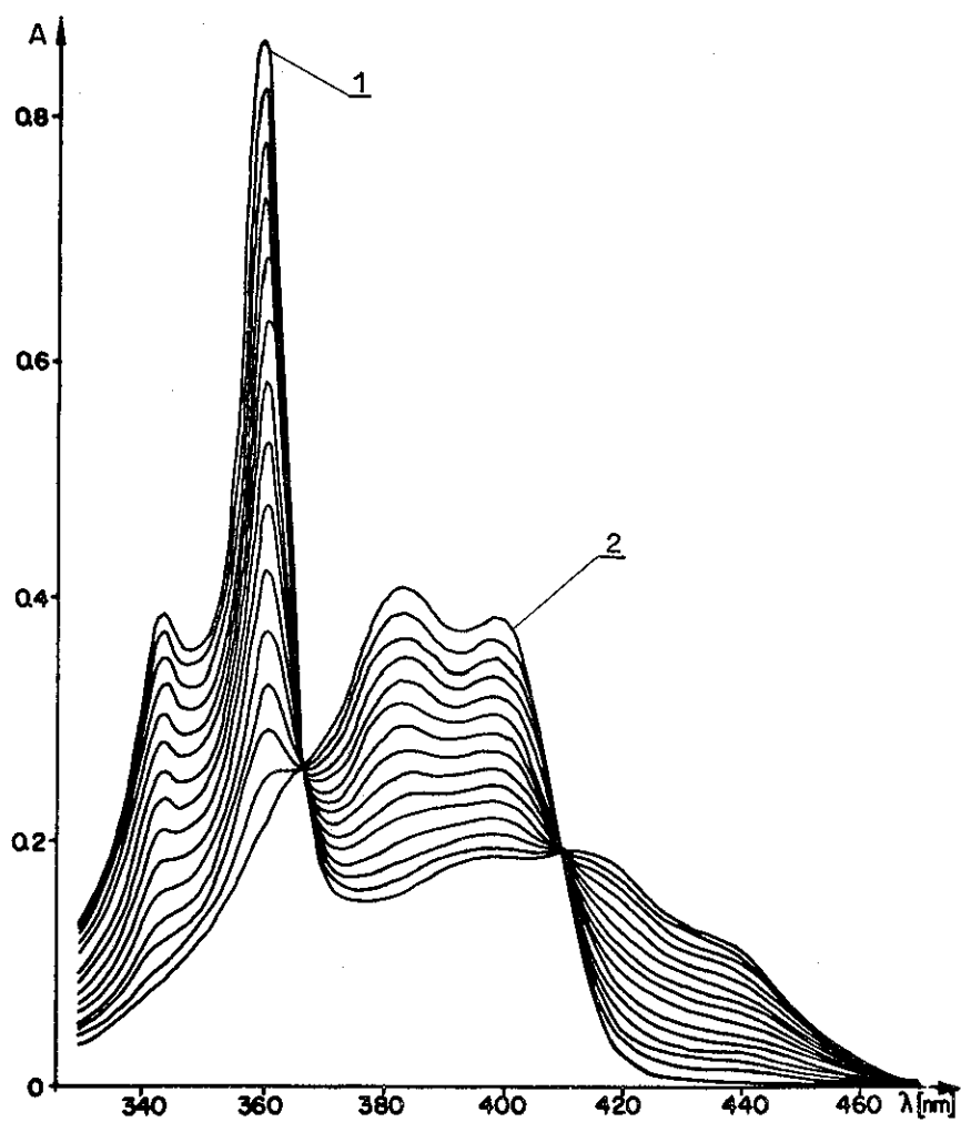
Figure 1. Absorption spectra of the reaction mixtures in solvolysis of 9-chloroacridine in 80 % acetic acid with 0.01 mm quartz cell. 1. 9-Chloroacridine, 1 m mole \times dm ^{-3} , 2. 9-acridanone.
