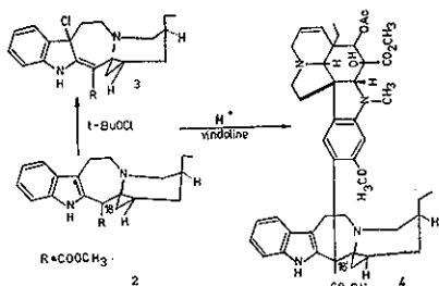
Figure 1. The coupling of 18β-carbomethoxy-4β-dihydrocleavamine (2) via its chloroindolenine intermediate 3, with vindoline.
