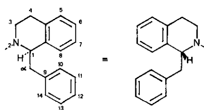
(R)-configuration
