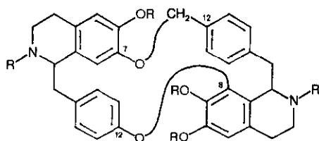
Group 12 * -8 * [7-12]
