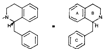
(S)-configuration
