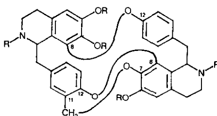
Group 8 * , 12 † -8 † , 12 * [11-7]
