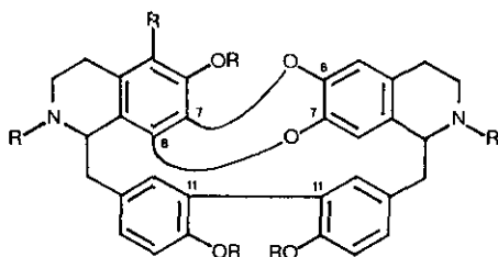
Group 7^*, 8^+ - 6^*, 7^+ (11-11)
