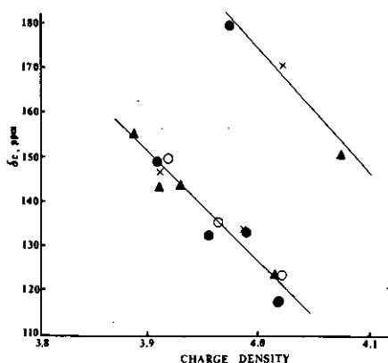
Fig. 2. Observed ^{13}\text{C} shieldings for uncoordinated pyridine (o), complexes 2d (•), 3d (▲), and 4d (x) vs. the calculated charge densities, the upper straight line referring to the quaternary carbons bonded to palladium and the lower one to the other ring carbons.
