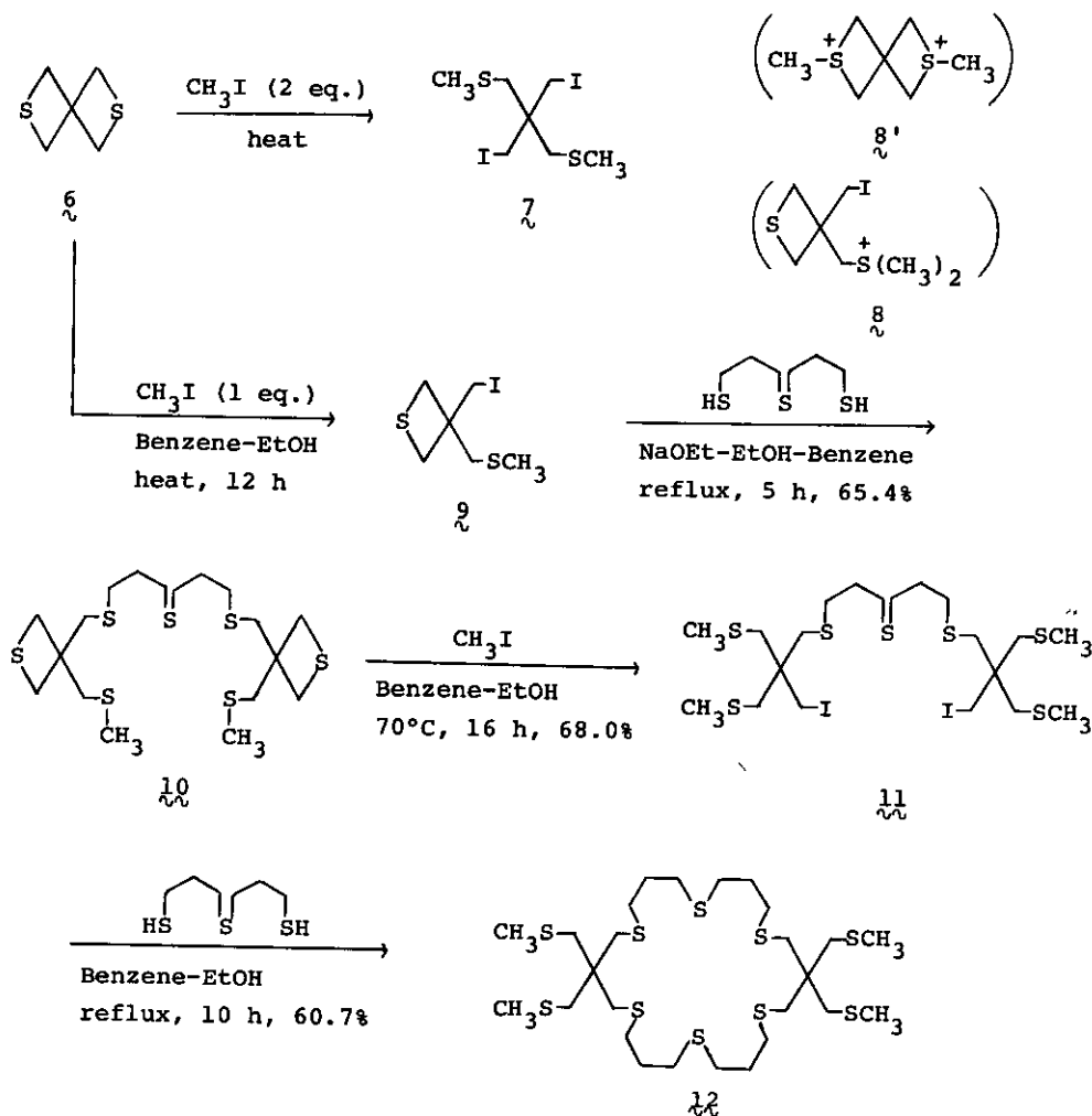
Scheme II
