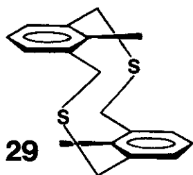
29 anti -isomer; \delta_{\text{CH}_3} = 1.30
