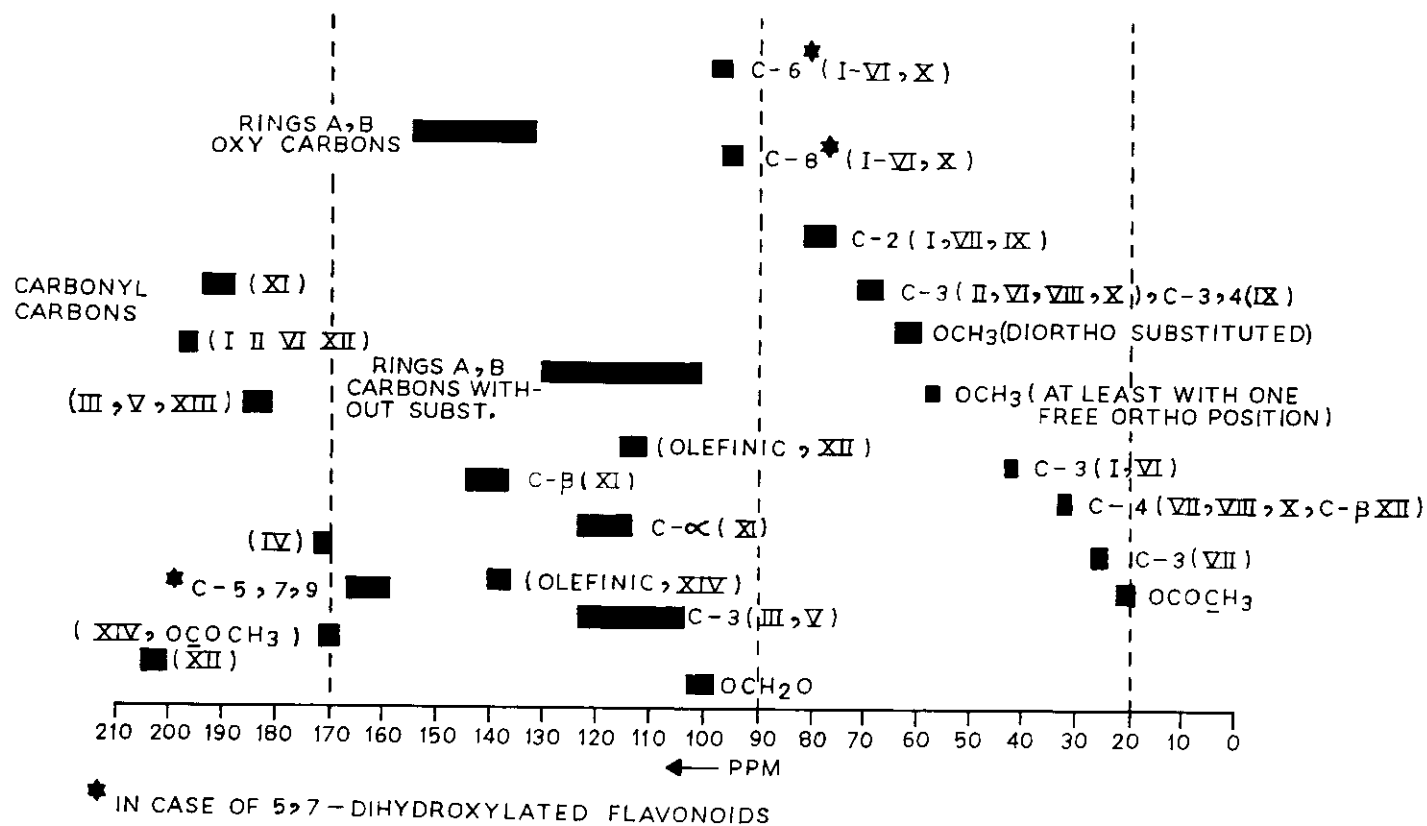
FIG. 2 CHARACTERISTIC SPECTRAL REGION IN CASE OF FLAVONOIDS AND RELATED COMPOUNDS
