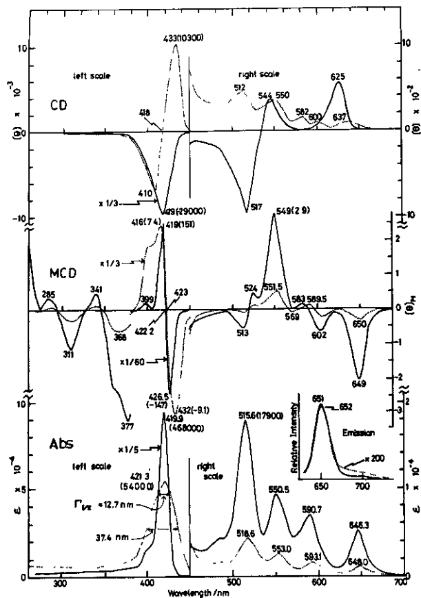
Fig.1 Absorption(bottom), MCD(middle), CD(top), and emission(inset) spectra of \text{I}_{\text{V}} in DMSO(—) and in 0.05 M TRIS buffer(pH 7.3)(- - - -) at 23±1 °C. Concentrations; 3.72 \times 10^{-5} M in DMSO except that in emission spectrum( 1.46 \times 10^{-4} M), and 1.46 \times 10^{-4} M in water. Taking into account of the aggregation problem cells were changed from 1 to 100 mm length keeping concentrations constant. In emission spectra, excitation was at 467 nm. Magnetic field; 11700 gauss. In order to maximize signal to noise ratio, all spectra are the average of at least triplicate runs, the cells being reversed in the second run. Unit; [\theta]_{\text{M}} = \text{deg cm}^2 \text{dmol}^{-1} \text{G}^{-1} . [\theta] = \text{deg cm}^2 \text{dmol}^{-1} .
