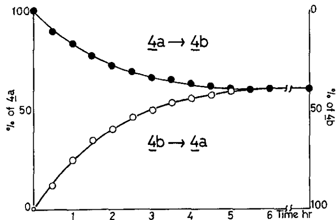
Figure 1. Rate of isomerization. \underline{4a} \rightleftharpoons \underline{4b} in dioxane at 80 °C.
