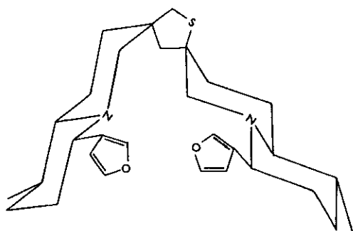
98 Thionuphlutine B
