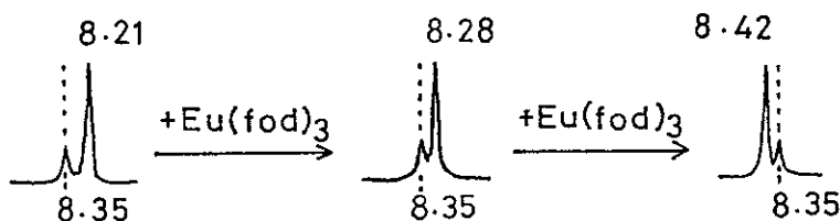
Fig. 1. ^1\text{H} Nmr study of the compounds ( 2b and 2c ) by using \text{Eu}(\text{fod})_3
