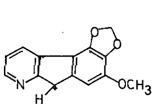
(c) m/z 240
