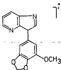
(a) m/z 268
