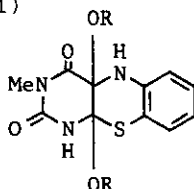
(4) a : R = Me b : R = Et c : R = n-Pr
