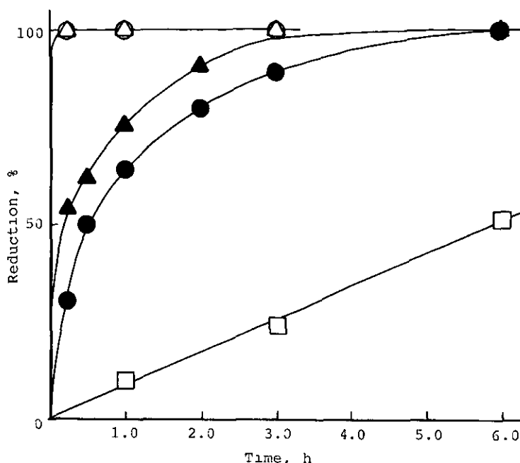
Fig.1 The Reduction of 1,2-Butylene Oxide with Lithium Borohydride in the Presence of Various Mole % of Triethylborane in Tetrahydrofuran at 25°C, [LiBH 4 ]=[Butylene oxide]=0.25 M. LiBH 4 /BET 3 ; 1/1 (○), 1/0.25 (△), 1/0.10 (▲), 1/0.05 (●), 1/0.00 (□).
