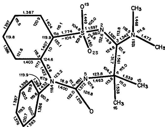
Fig. 1. Molecular structure of the 4,5,6,7-tetrahydro-1,2,5,7-benzothiatriazin-6-on-1,1-dioxide 7 .
