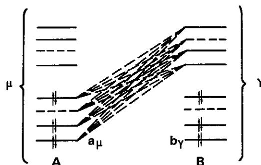
Figure 4.2. The interaction between \mu and \nu molecular orbitals (the term \text{occ.a} \quad \text{unocc.b} )
