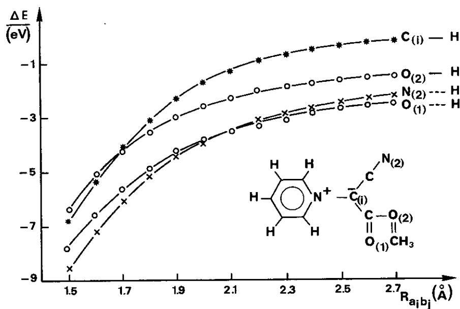
Figure 4.4. The variation of \Delta E versus R_{a_1b_j} in reaction between cyanoamidyropyridinium methylyde and hydronium cation.
