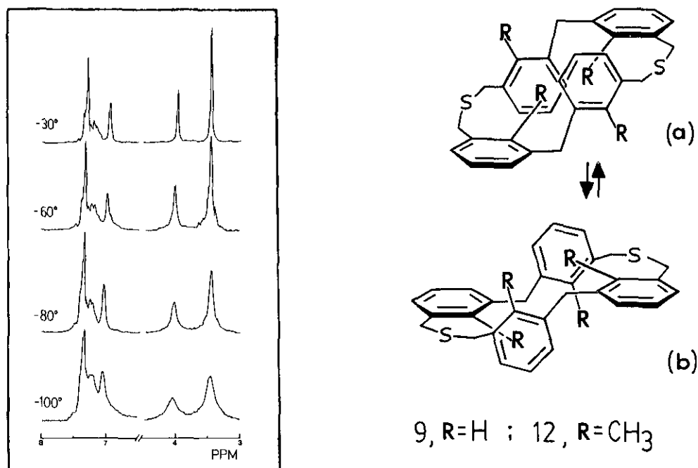
FIGURE 1. Variable temperature ^1\text{H} -NMR spectra [ \text{CDCl}_3/\text{CD}_2\text{Cl}_2 (1:1); 90 MHz] of the dithia[3.1.3.1]metacyclopentane 9 .
