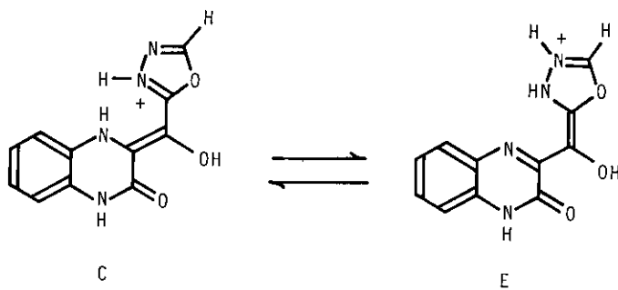
SCHEME 39 Equilibria of 32 in TFA
