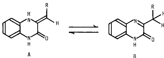
SCHEME 3 Equilibria of 1 in DMSO- d 6 or TFA
