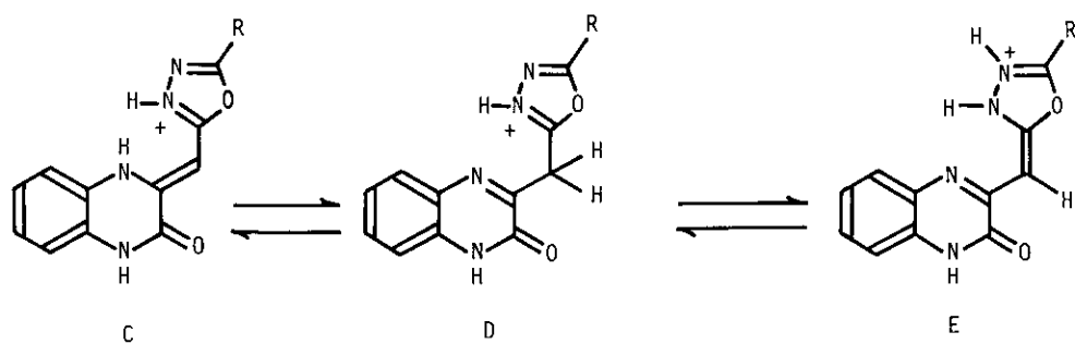
Compound 30a 30b 35 SCHEME 37 Equilibria in TFA
