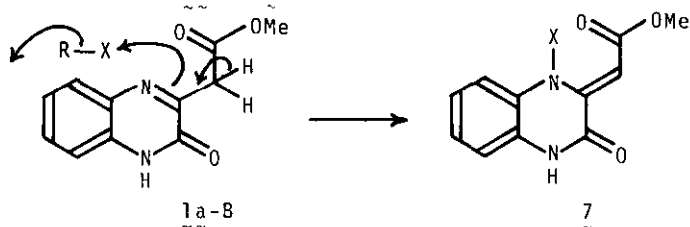
(a) mechanism from 1a to 7
